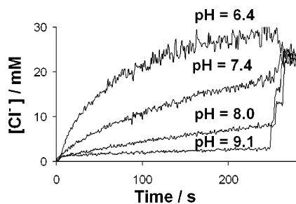
Figure 4. Transmembrane Cl - transport by 2 as a function of pH. Experiments were done using EYPC liposomes with lucigenin (1 mM) in a 100 mM NaNO 3 /10 mM sodium phosphate buffer at various pH. Compound 2 was added to give a 2:100 ligand/lipid ratio. At t = 0 s, NaCl solution was added to give an external Cl - concentration of 25 mM. Lucigenin fluorescence was converted to Cl - concentration using the Stern–Volmer constant determined under the assay conditions. All traces shown are the average of three trials.
